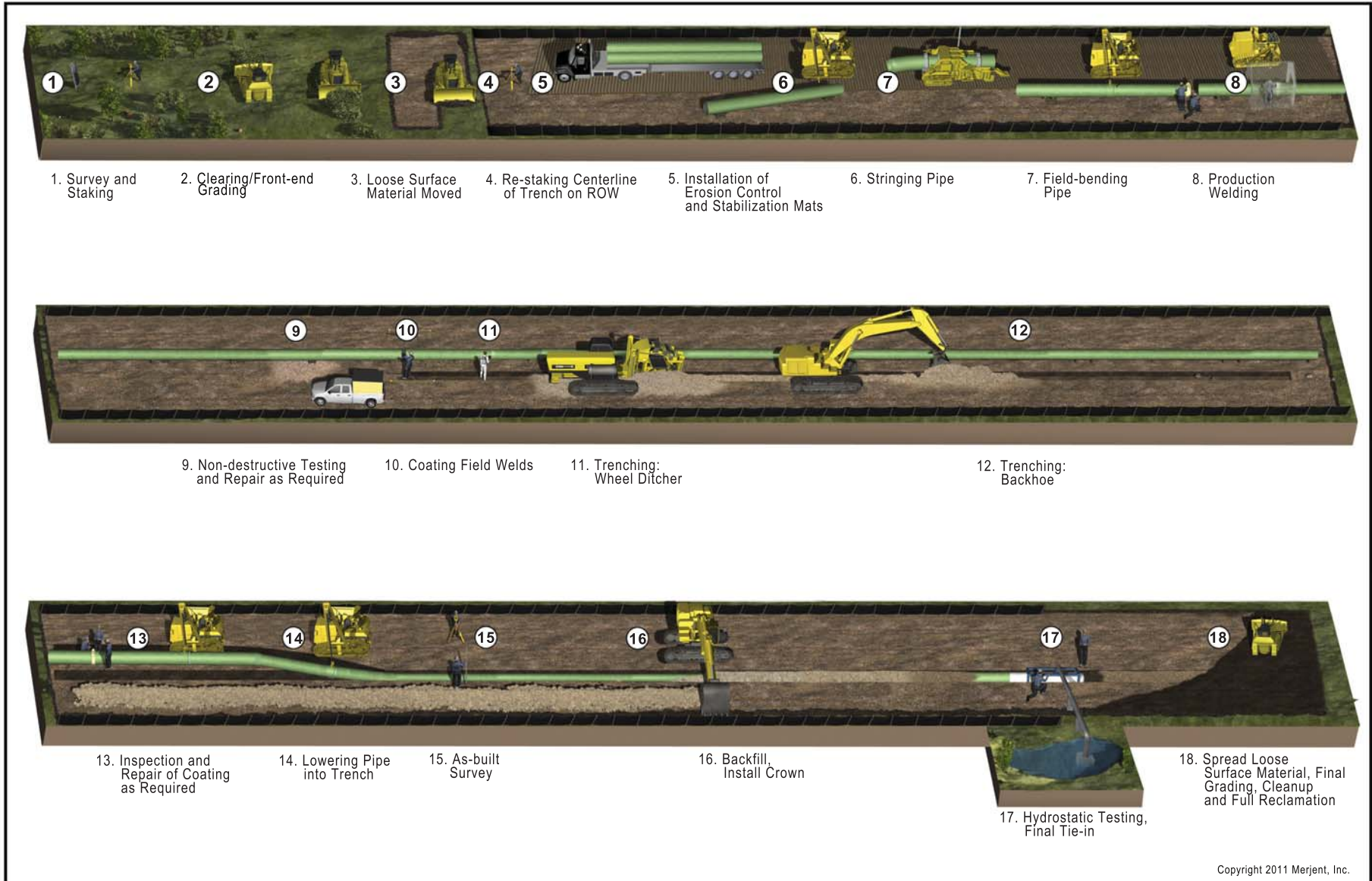
Figure 4.3-1 Line 5 Wisconsin Segment Relocation Project Typical Construction Sequence
