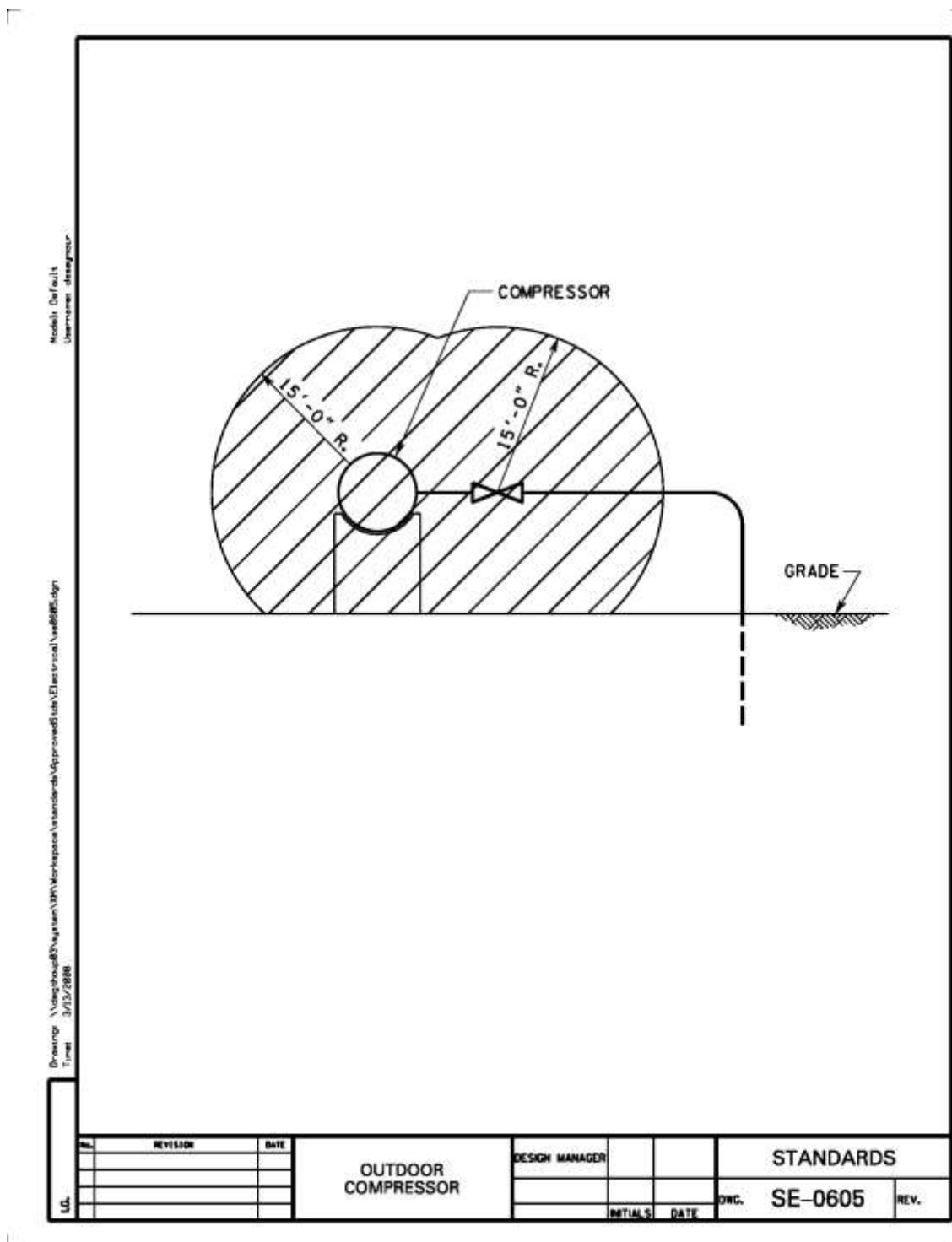
Figure 16: Outdoor Compressor
