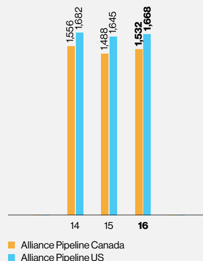
Alliance Pipeline – Average Throughput Volumes (millions of cubic feet per day)
